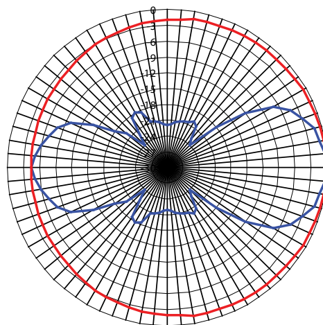
RADIATION PATTERN
