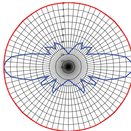
RADIATION PATTERN
